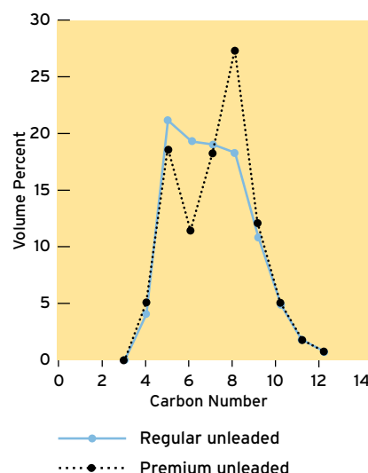
Gasoline Carbon Number Distribution
