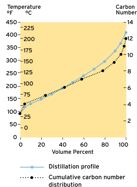
Distillation Profile vs. Cumulative Carbon Number Distribution
