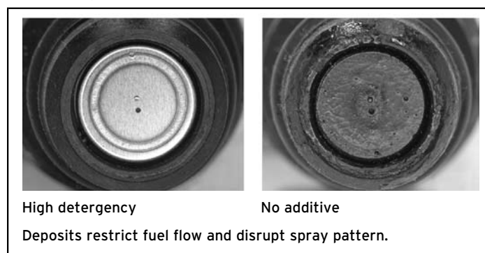
Port Fuel Injector Director Plate Deposits
