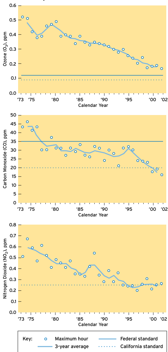
Maximum Hourly Pollutant Levels in California 1973-2002
