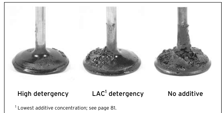
Typical Intake Valve Deposits
