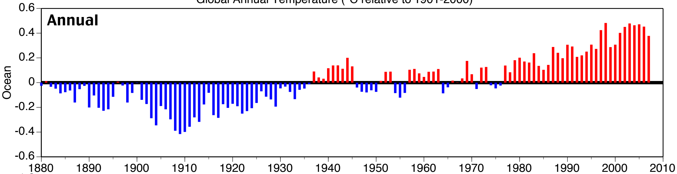
Global Annual Temperature ( ^{\circ}\text{C} relative to 1901-2000)
