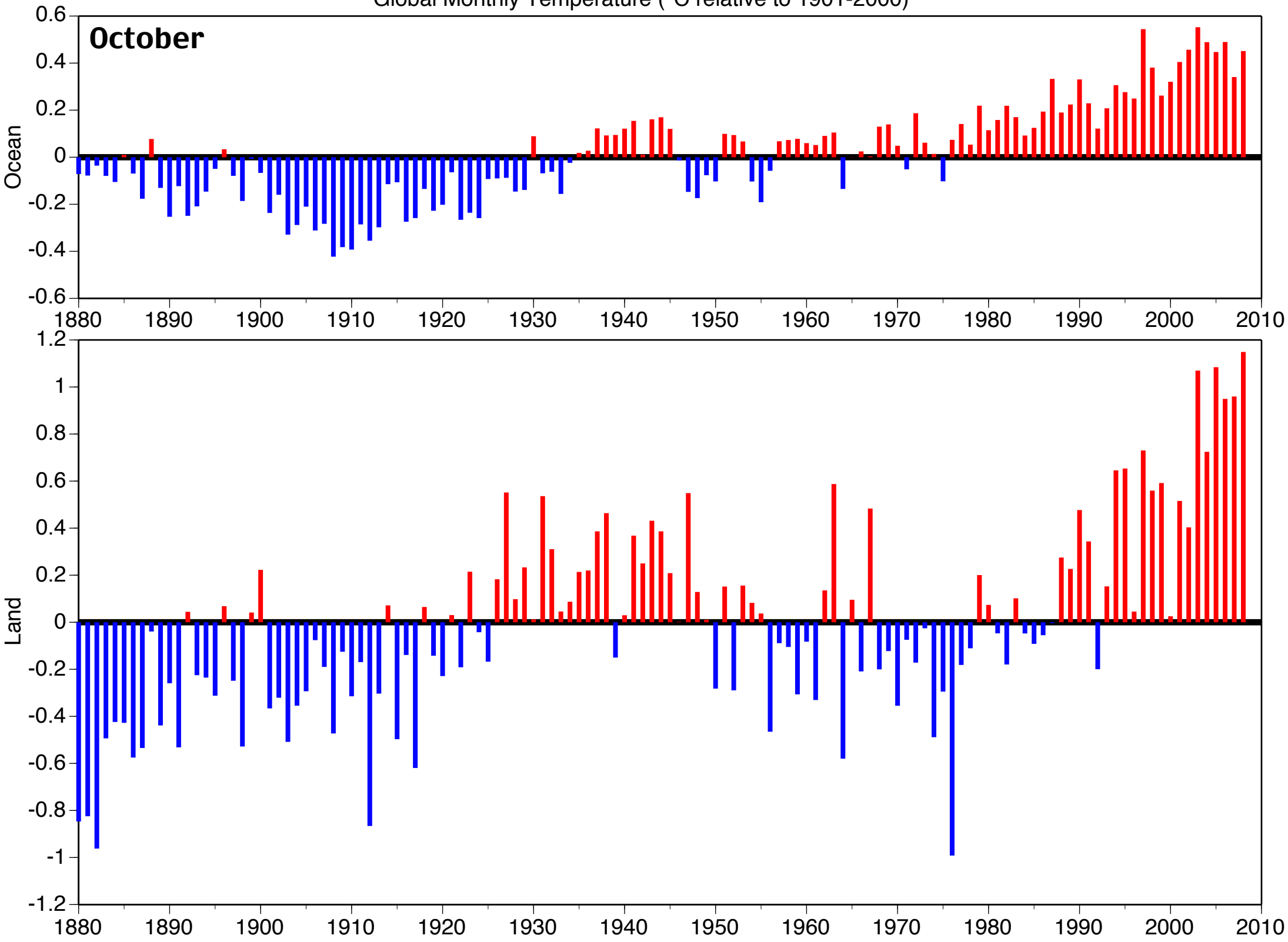
Global Monthly Temperature ( ^{\circ}\text{C} relative to 1901-2000)
