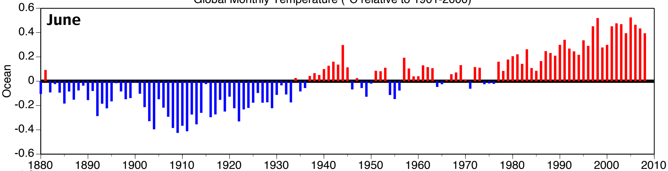
Global Monthly Temperature ( ^{\circ}\text{C} relative to 1901-2000)
